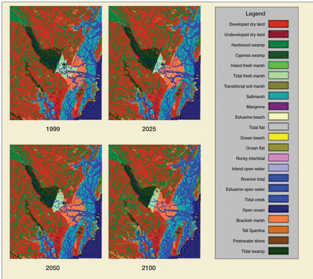
Figure 2. SLAMM simulation of effects of accelerated SLR on tidal marshes of the Altamaha River, Georgia. The simulation was run using the SRES A1B scenario that assumes a 52-cm increase in sea level by 2100. The coarse vertical resolution of the NED dataset results in the linear pattern (ie striping) of wetland migration observed during the simulation.
