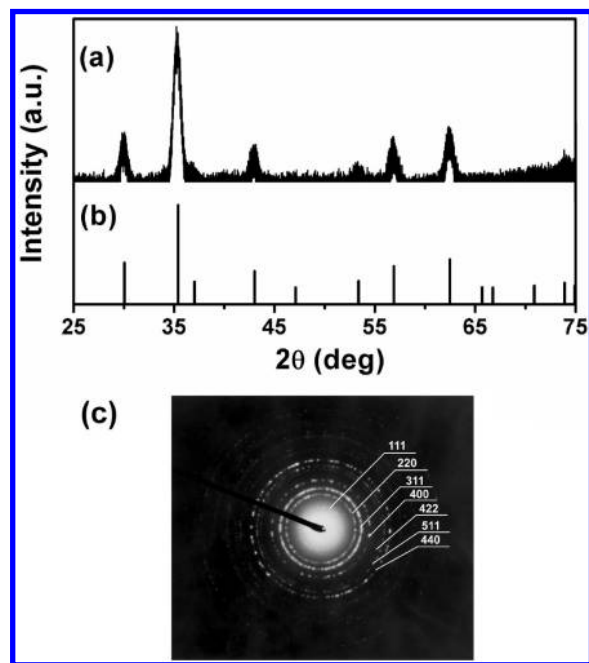
FIGURE 1. (a) X-ray diffraction patterns of \text{MnFe}_2\text{O}_4 NPs having an XRD-estimated average grain size of 10.6 nm at room temperature, (b) the JCPDS card data of \text{MnFe}_2\text{O}_4 (No. 10–0319), and (c) selected-area electron diffraction (SAED) of \text{MnFe}_2\text{O}_4 NPs.
