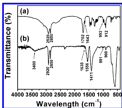
FIGURE 3. FTIR spectra of (a) pure 16-heptadecenoic acid and (b) surfactant-modified \text{MnFe}_2\text{O}_4 NPs.
